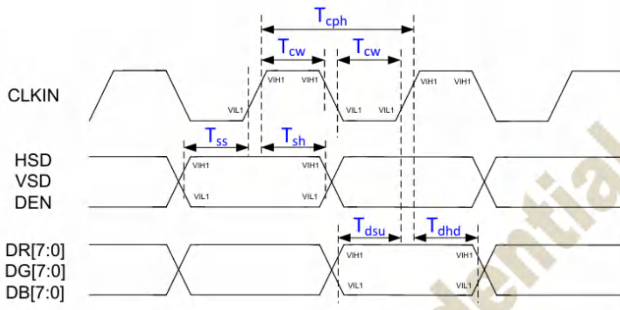
Figure: Input signal timing
